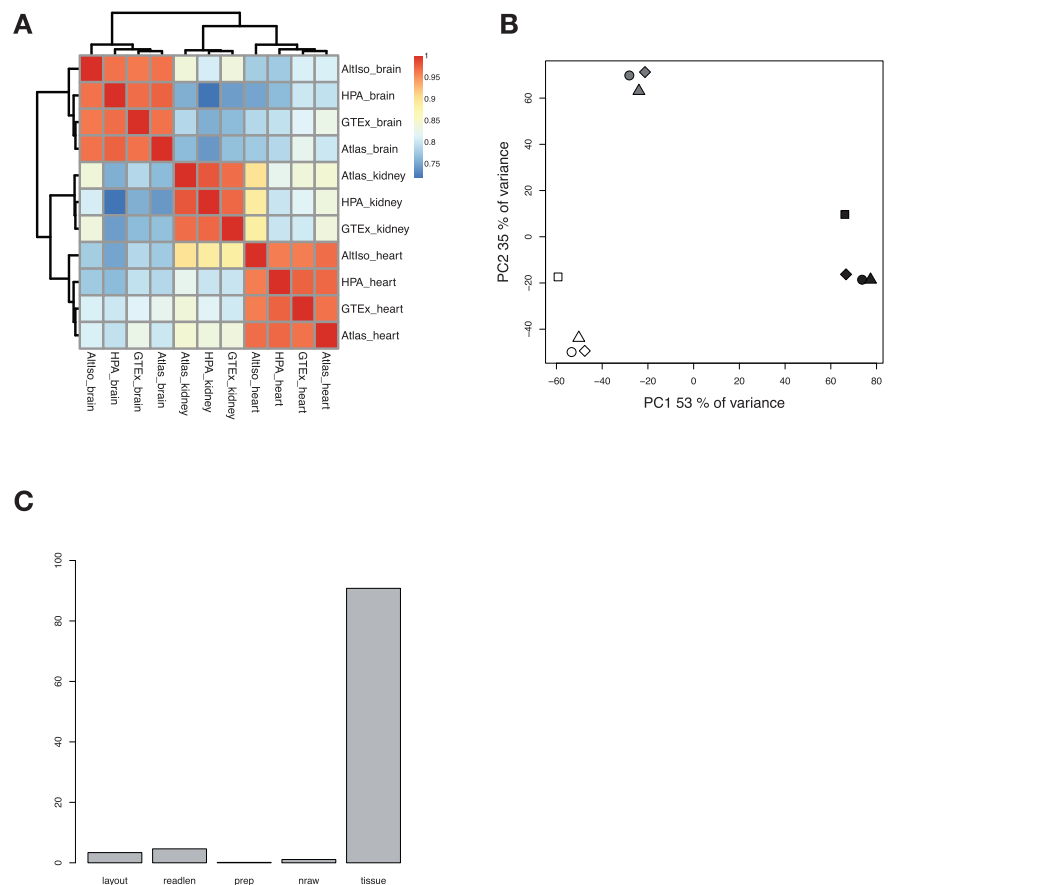
Figure 3. Analysis of precomputed FPKM/RPKM ( n = 13,078 ) values for brain, heart and kidney samples from four different studies after removal of batch effects using ComBat. In the principal component plot, tissue types are indicated with white (heart), black (brain) and grey (kidney). Studies are indicated with different symbols; circle (HPA), square (Altiso), diamond (GTEx) and triangle (Atlas). (A) Heat map with Spearman correlations between samples. (B) PCA, PC1 and PC2. (C) ANOVA dependence of the laboratory factors layout, read length, preparation, number of raw reads and tissue.
